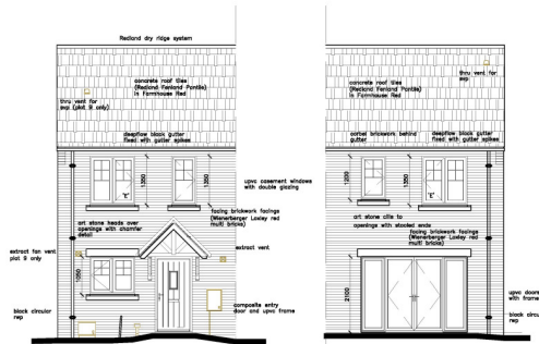
Approach Elevation
