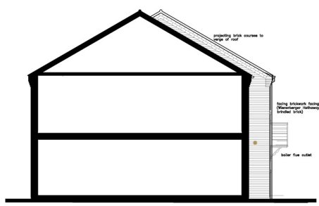
Gable Elevation (plot 9)
