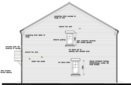
Gable Elevation (plot 10)
